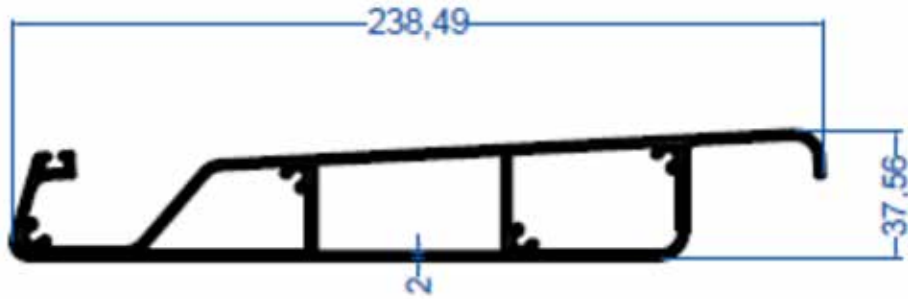
PANEL PROFİL
