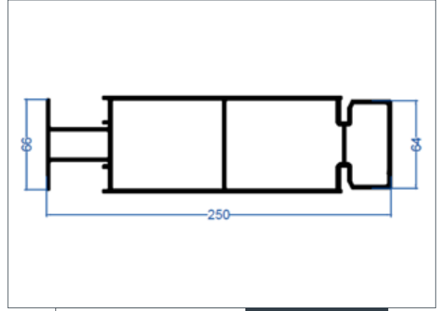
ANA RAY
