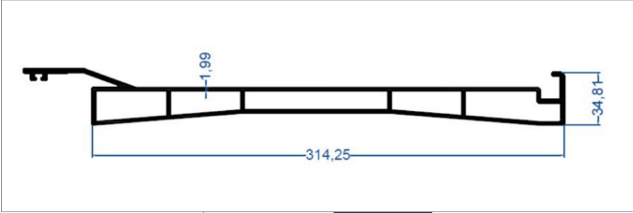
PANEL PROFİL
