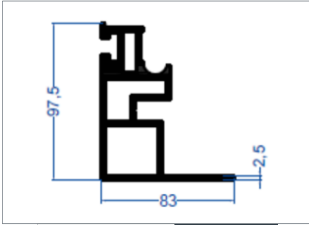
ALT RAY
